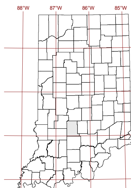
Index map of Indiana showing the location of Monroe County
