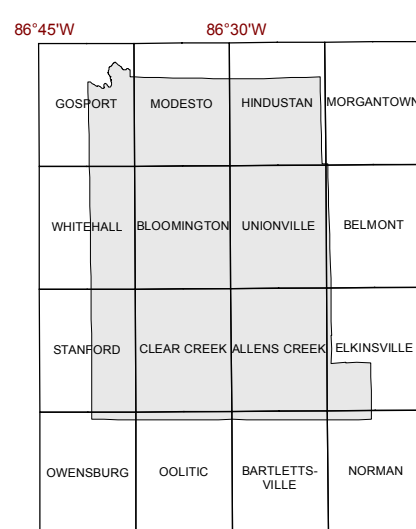
Index map of Monroe County showing U.S. Geological Survey 7 1/2-minute topographic quadrangle map names
